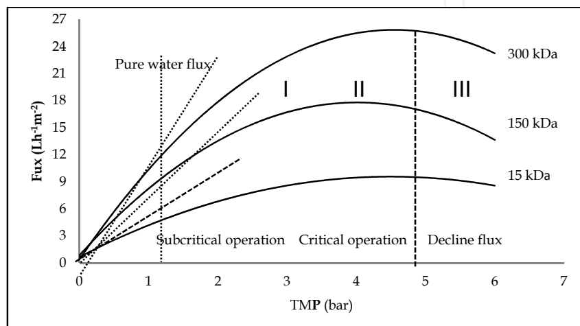
Fig. 6. Critical flux regimes in membranes of 300, 150 and 15 kDa: (I) Subcritical operation (II) Critical operation (III) Decline flux.
