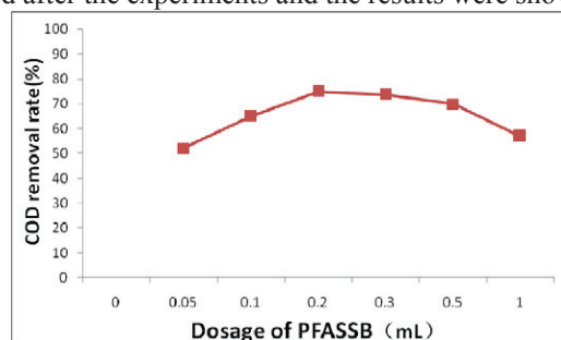
Figure 2. COD removal at different dosage of flocculant
